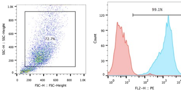
Figure: Characterization of CD40 overexpressing in 293T stable clones using FACS.
